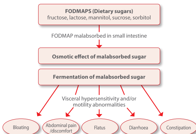
Figure 1: Mechanism of functional gut symptoms related to FODMAP ingestion.
